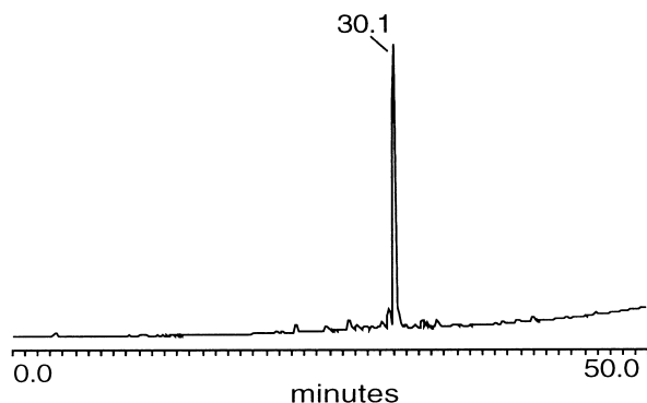
Figure 1. RP-HPLC analysis of reduced octreotide. Sample was taken from the extraction (20% acetic acid solution). The retention time was 30.1 as monitored at UV 214 nm. The elution: A=5% acetonitrile aqueous containing 0.1% TFA; B=90% acetonitrile aqueous containing 0.1% TFA. See Experimental for HPLC conditions.
