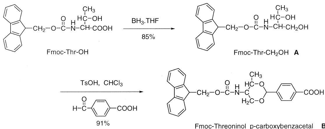
Scheme 1. The synthesis of Fmoc-threoninol p -carboxybenzactal B .
